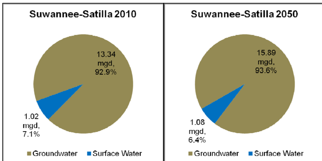
Figure 8: Baseline Industrial Water Demand by Source
